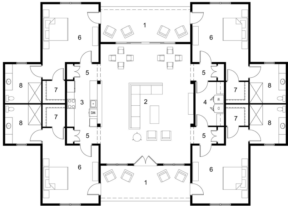
FLOOR PLAN 1/16" = 1'
